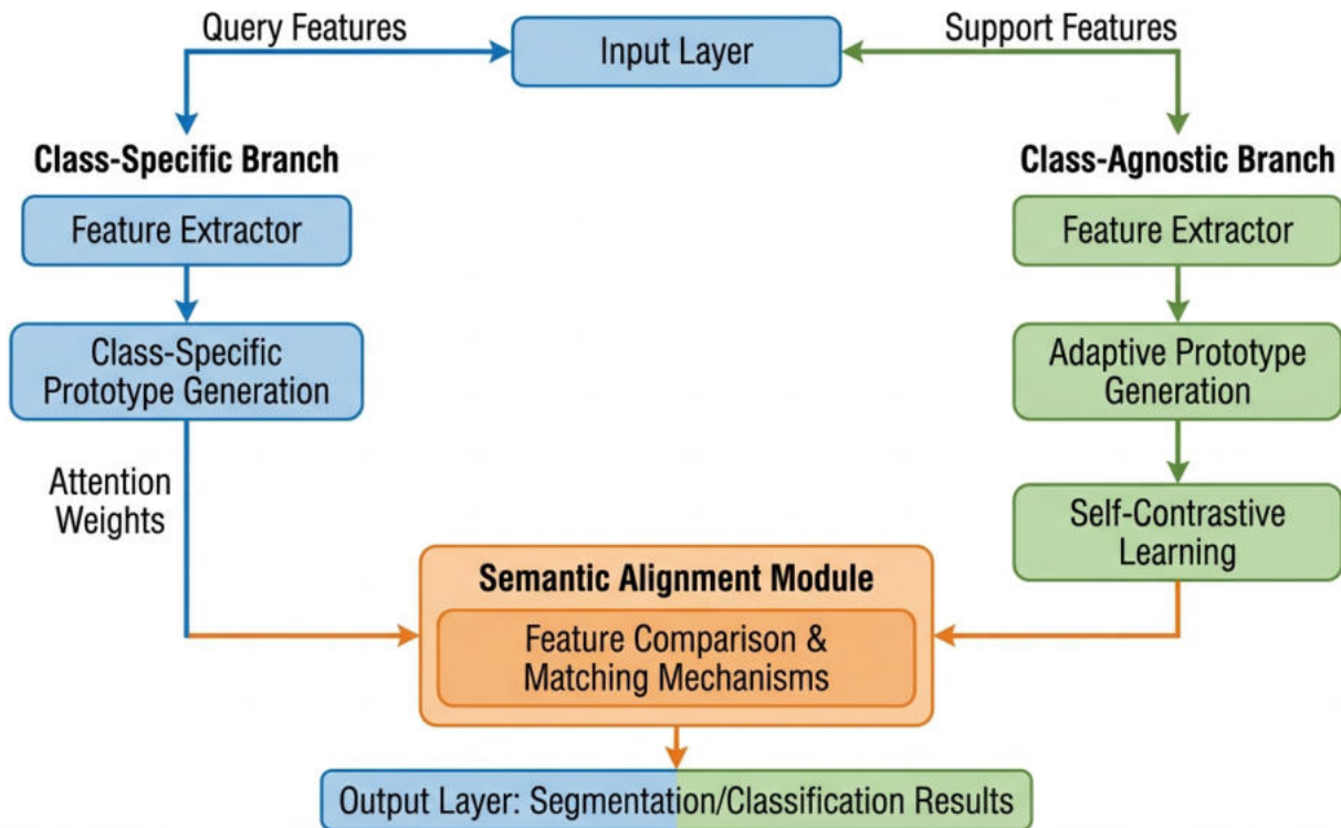
Figure 1: Architecture Diagram of Adaptive Prototype Attention (APA) Model
